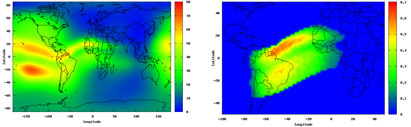
Figure 2: TEC (left panel) and scintillation map (right panel) obtained by modeling
