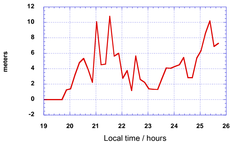
Figure 8: Positioning error at Naha (Japan) under scintillation conditions, computed with GISM
