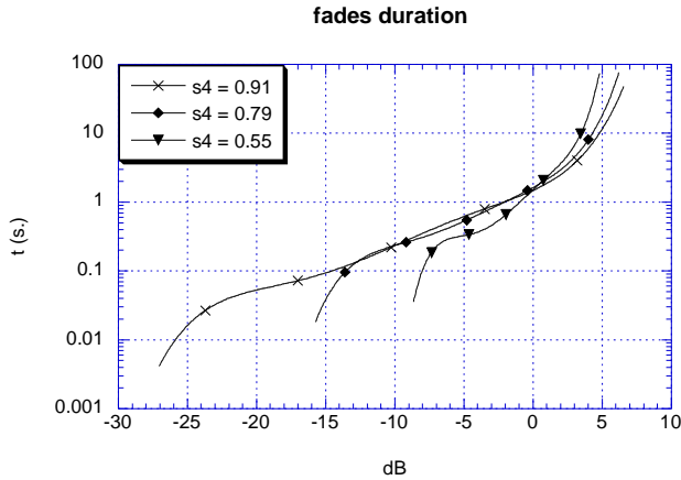
Figure 6: fades duration vs fade depth
