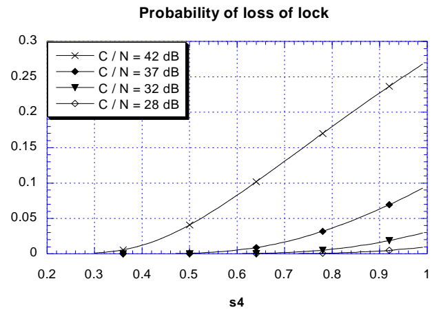
Figure 7: Probability of loss of lock
