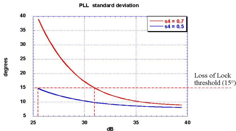
Figure 5: PLL standard deviation vs C/N_0
