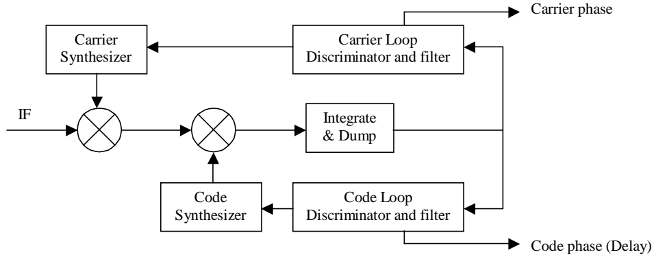
Figure 3: Simplified GPS Digital Receiver Channel
